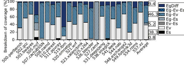
Fig. 15: Coverage breakdown by predictors.
