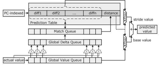
Fig. 1: The structure of the gDiff value predictor. [37]
